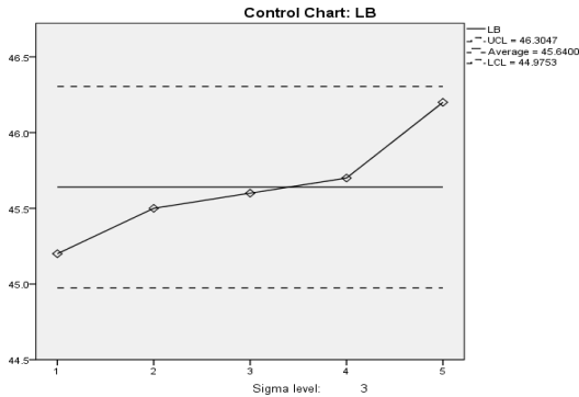
Gambar 2 Grafik Control Chart Lebar Bahu
